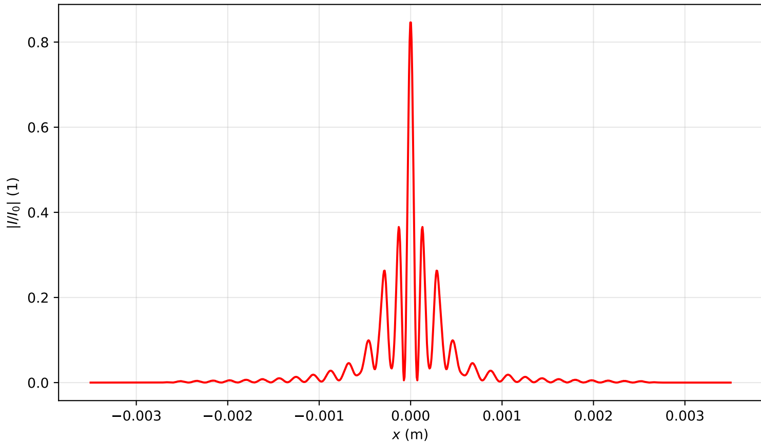
Intensity profile I(x, y = 0, z = 0.159)/I_0 , \text{Pin}=9.0\text{Pcr} , artificial time
